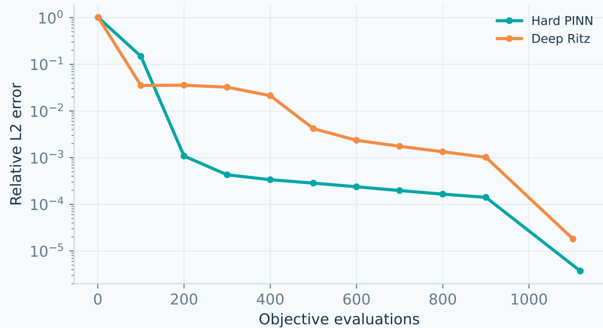
Independent validation during training
