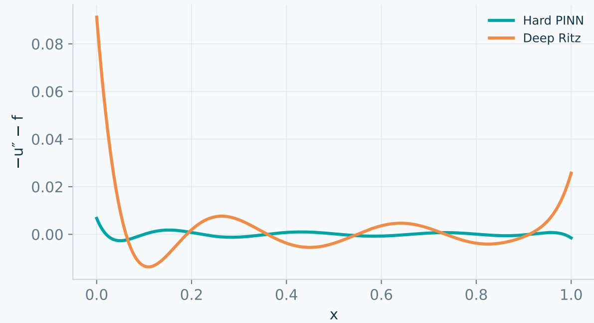
Physical residual on a fresh grid
